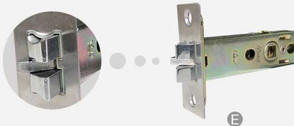
Standard 60mm Single Latch E with Anti-prying Tongue
